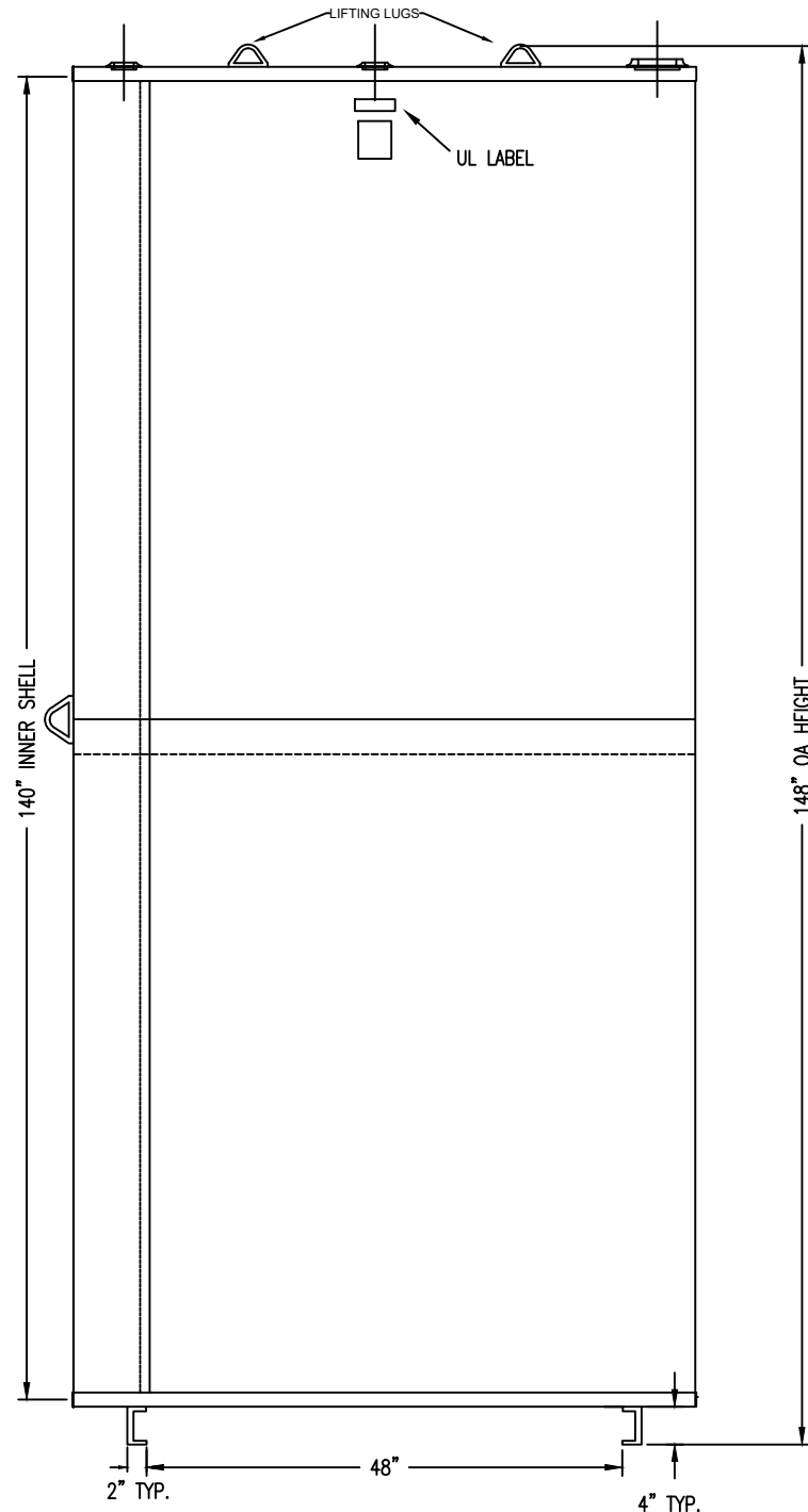
FRONT VIEW
