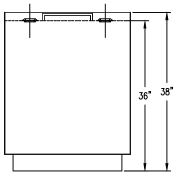
LEFT VIEW
