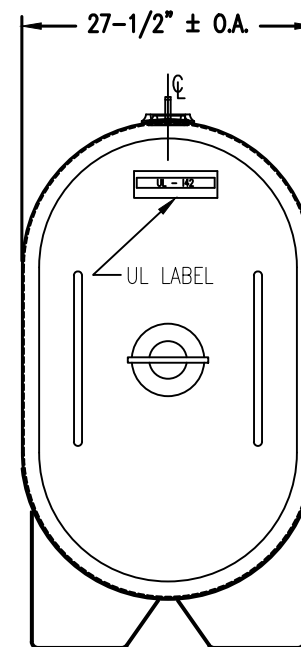
END VIEW
