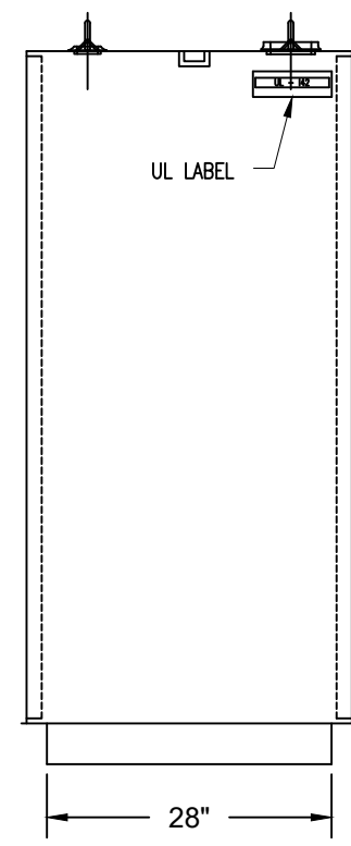
RIGHT VIEW
