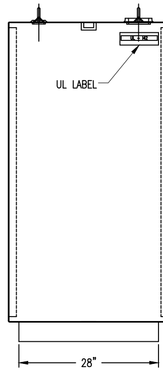
RIGHT VIEW
