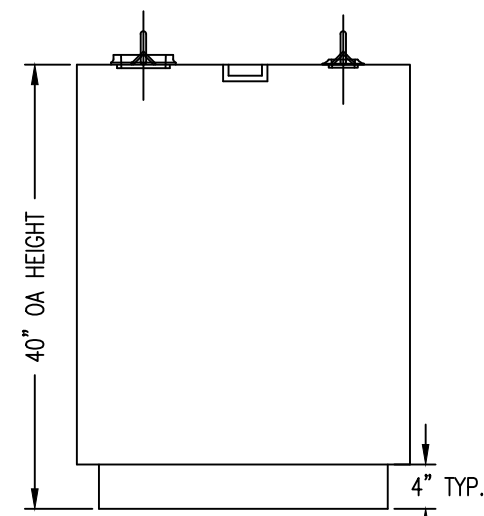
LEFT VIEW
