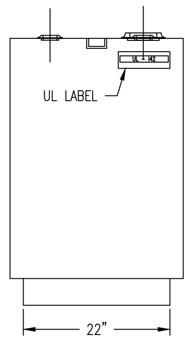
RIGHT VIEW
